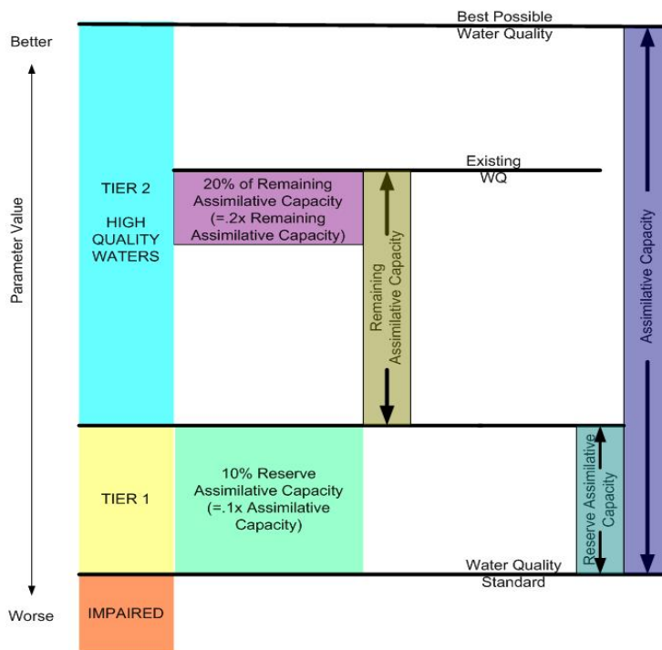
CONCEPTUAL DIAGRAM FOR TIER 1 AND TIER 2 WATERS ESTIMATION (not to scale)
